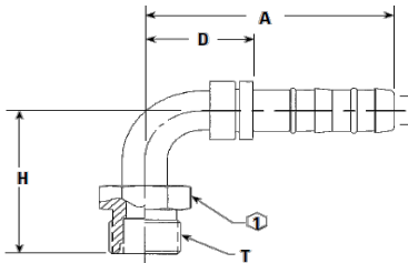
90° Male O-Ring (rigid) Metric Thread
