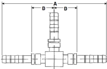
"T" Splicer - 3 Hose Connector
