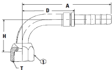
90° Female SAE 45° Flare To FlexCLIK Hose
